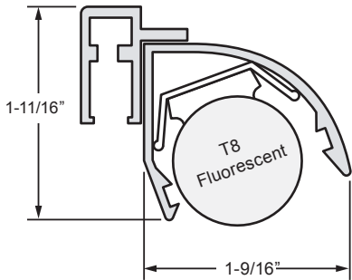
202/250 Rail/Lamp Shield
