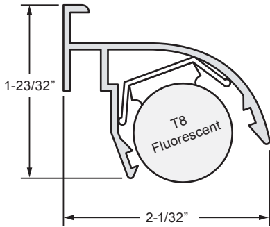
252 Lamp Shield
